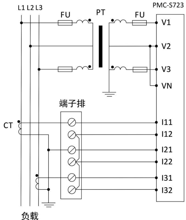
图 3-7 DELTA, 2CT
