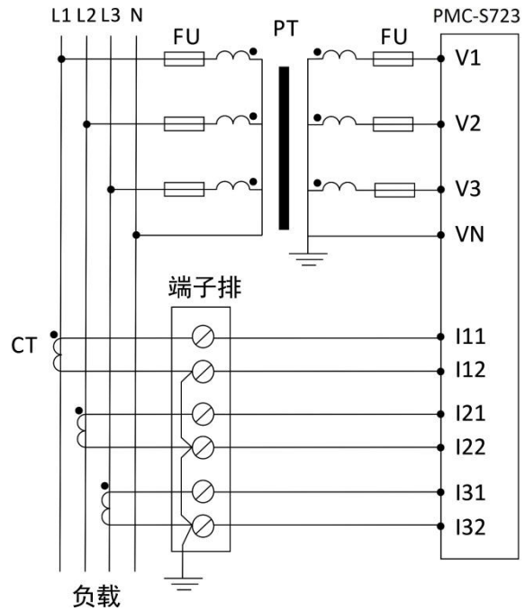
图 3-5 WYE, 3PT, 3CT
